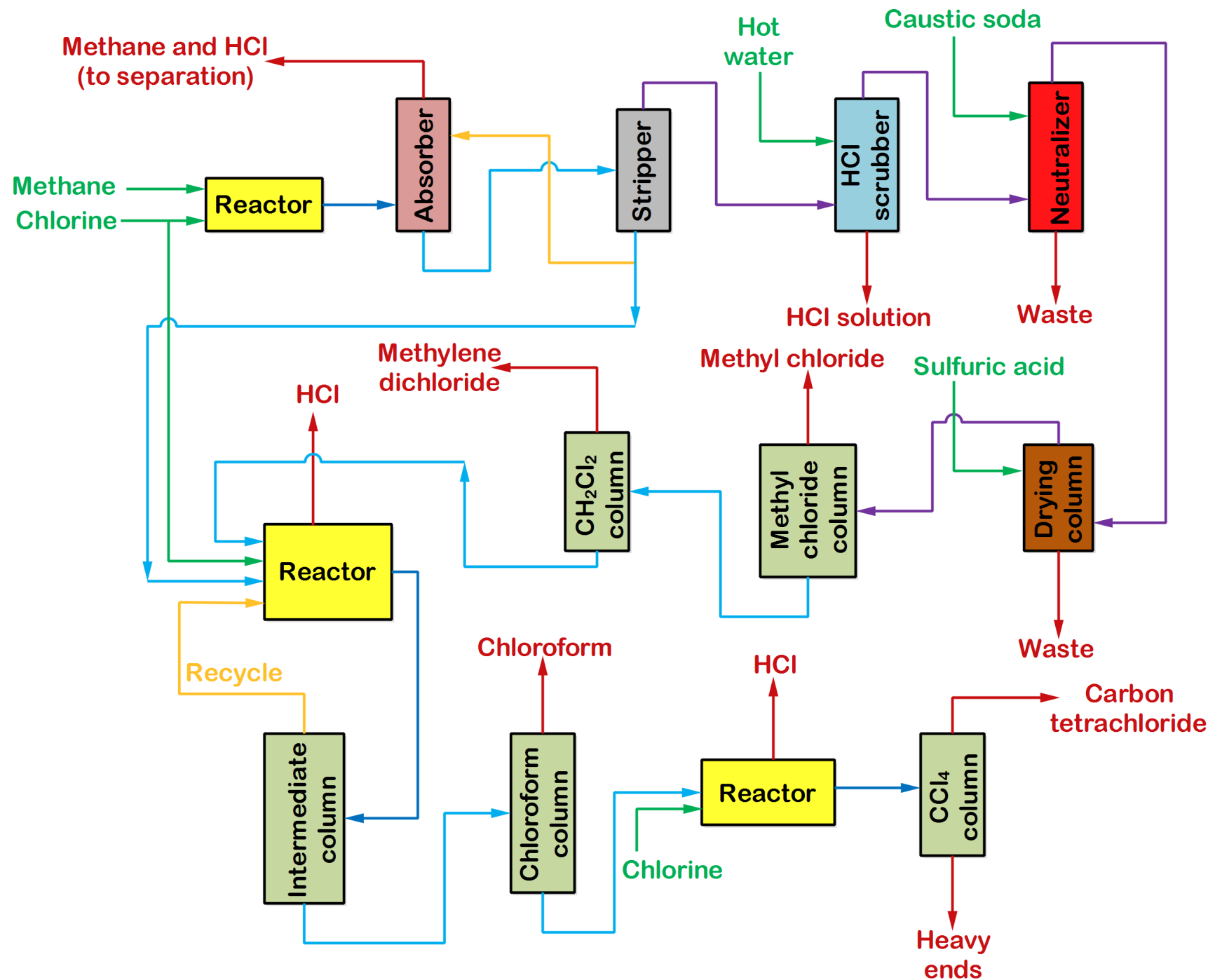
Figure: Manufacture of Methyl chloride, methylene dichloride, chloroform, carbon tetrachloride from methane by chlorination
